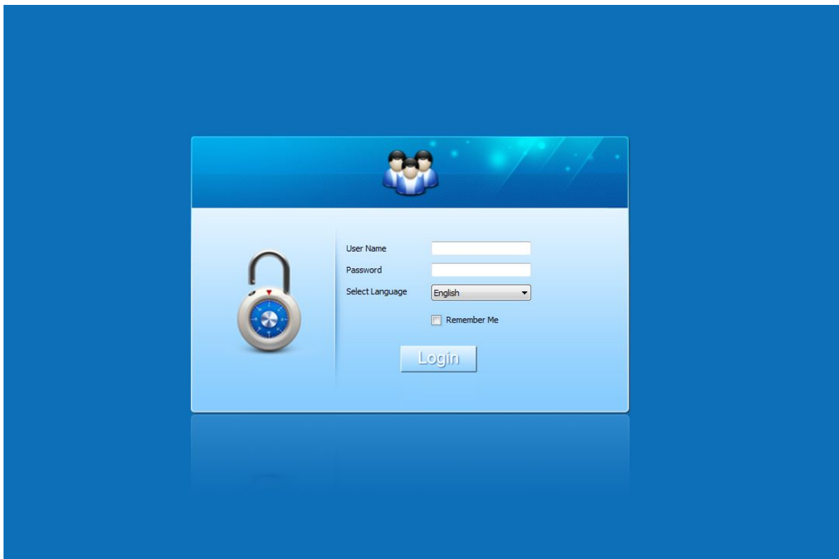
Figure3- 1 Login interface
